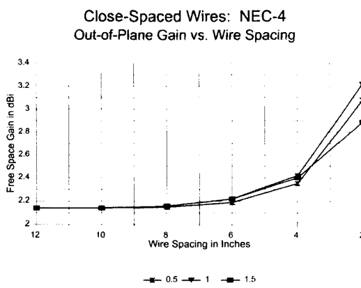
Figure 14—Out-of-plane gain of close-spaced wires— NEC-4 .
