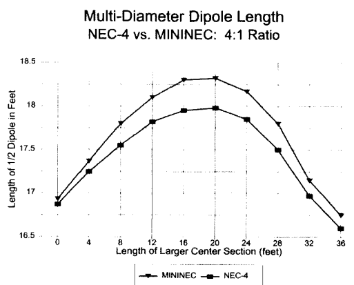
Figure 9—Multi-diameter dipole length— NEC-4 versus MININEC .
