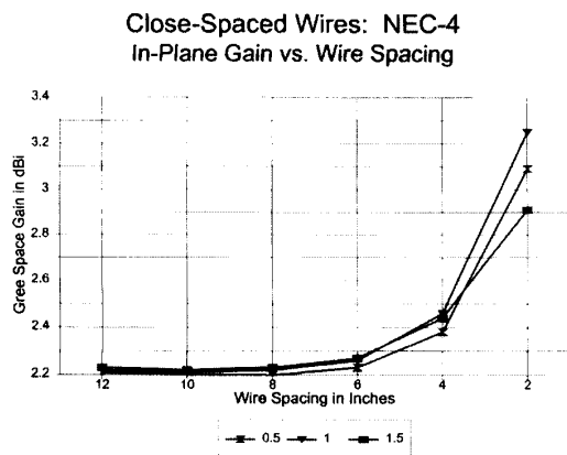
Figure 13—In-plane gain of close-spaced wires— NEC-4 .
