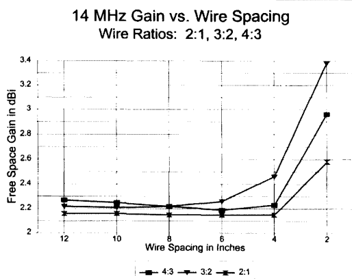
Figure 19—14 MHz gain versus wire spacing for different length ratios.
