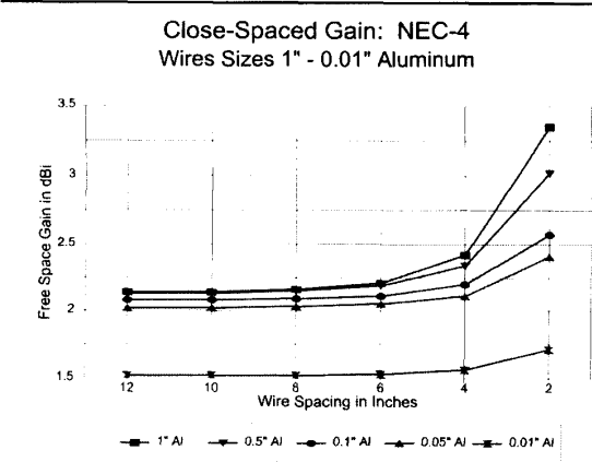
Figure 21—Close-spaced gain for wire sizes from 0.01 to 1.0 inch diameters— NEC-4 .
