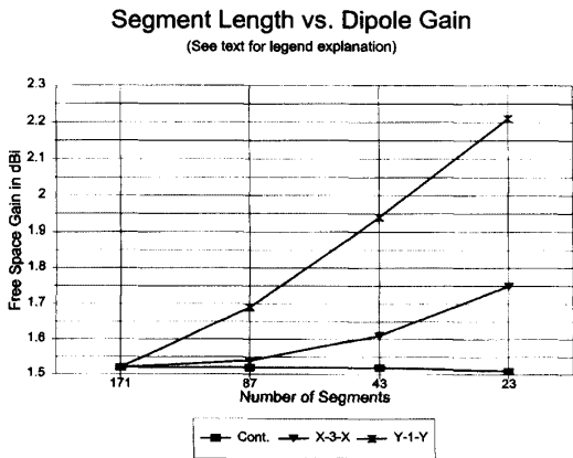
Figure 3—Segment length versus dipole gain for different methods of segmentation.
