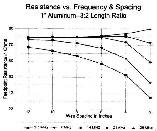
Figure 23—Feed-point resistance versus frequency and spacing.
