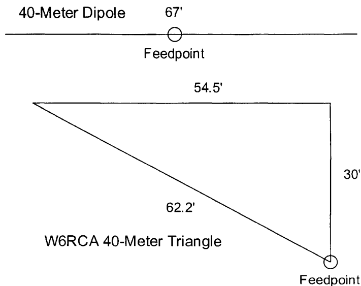
Figure 1—Two antennas for comparative convergence tests.
