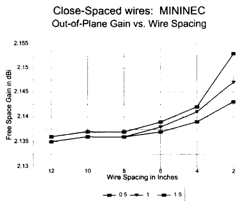
Figure 12—Out-of-plane gain of close-spaced wires— MININEC .
