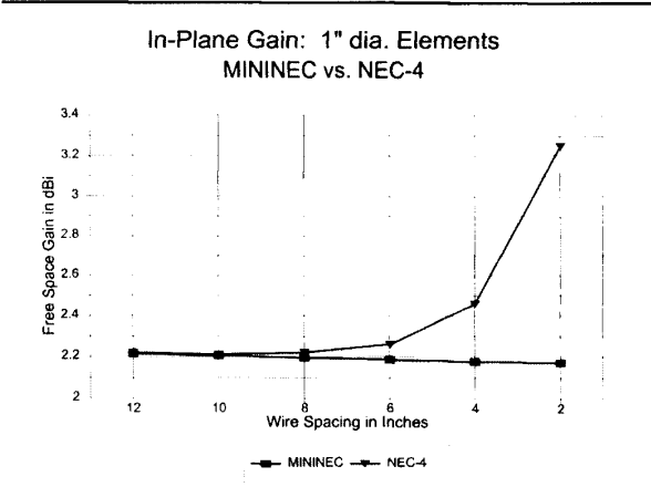
Figure 15—In-plane gain of close-spaced wires— MININEC versus NEC-4 .
