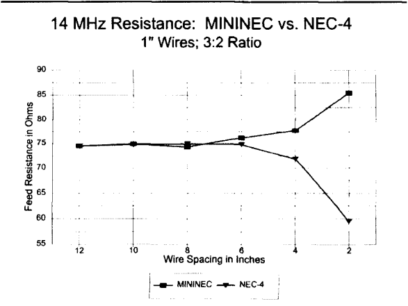
Figure 18—14 MHz resistance— MININEC versus NEC-4 .
