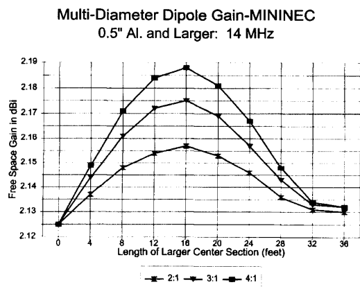
Figure 5—Multi-diameter dipole gain— MININEC .
