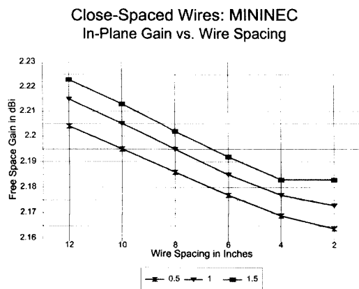
Figure 11—In-plane gain of close-spaced wires— MININEC .
