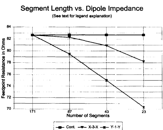
Figure 4—Segment length versus dipole impedance for different methods of segmentation.
