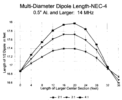
Figure 8—Multi-diameter dipole length— NEC-4 .
