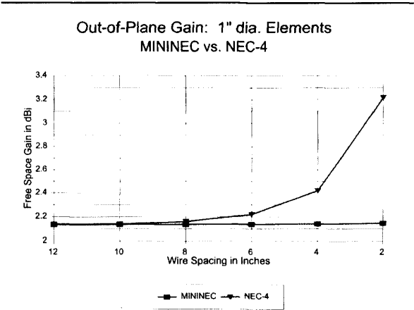
Figure 16—Out-of-plane gain of close-spaced wires— MININEC versus NEC-4 .
