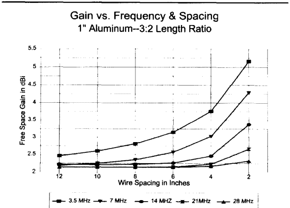
Figure 22—Gain versus frequency and spacing.
