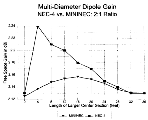
Figure 10—Multi-diameter dipole gain— NEC-4 versus MININEC .
