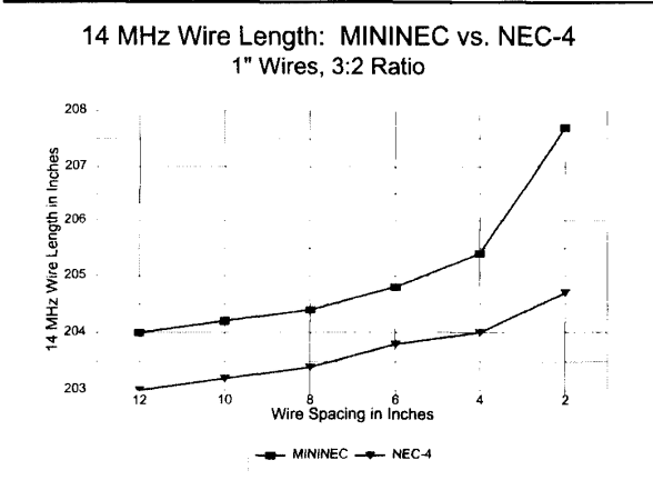
Figure 17—14 MHz wire length— MININEC versus NEC-4 .
