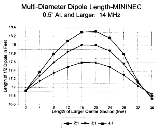
Figure 6—Multi-diameter dipole length— MININEC .
