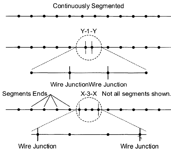
Figure 2—Three methods of segmenting a dipole.
