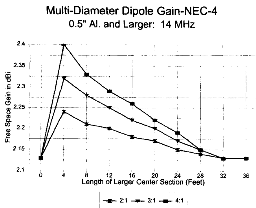
Figure 7—Multi-diameter dipole gain— NEC-4 .
